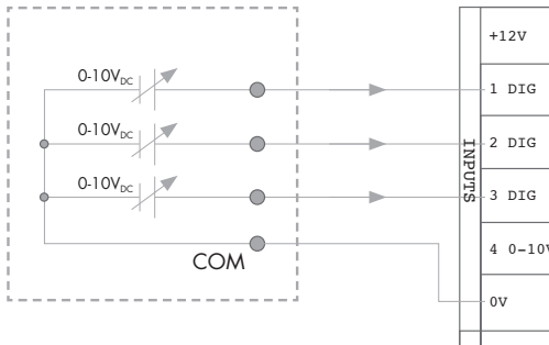
Externe sturing
